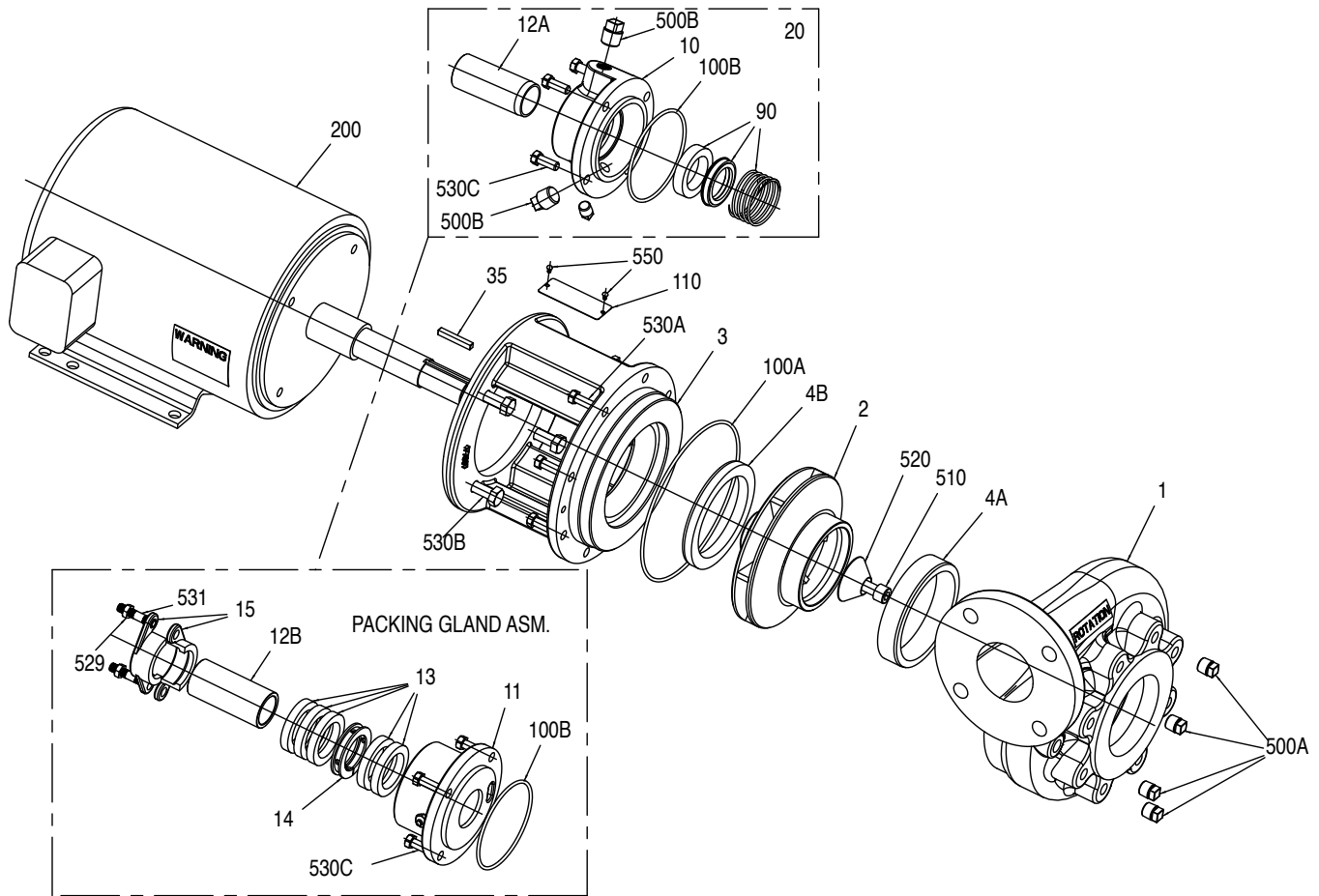
MECHANICAL SEAL ASM.
