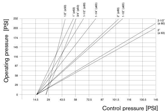
Control function B; Actuator 50 ° 80 mm
