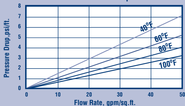
Pressure Drop
