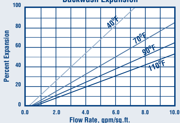
Backwash Expansion
