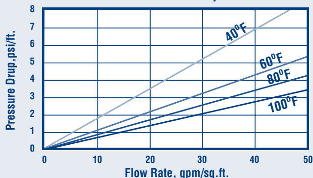
Pressure Drop
