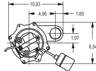
PFS411A with automatic float
