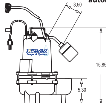
PFS411A with automatic float
