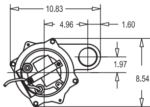
PFS411 & PFS421 without float
