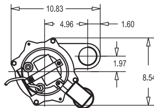
PFS411VF vertical level control with piggy-back plug
